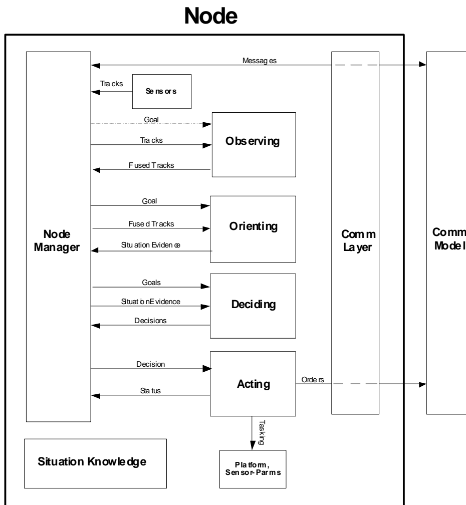
Figure 4 Internal OODA Structure of a Node.
