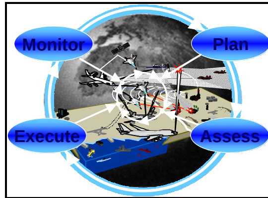
Figure 7: OODA Loop
