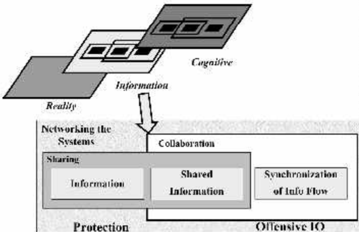
Figure 35. Information Elements
